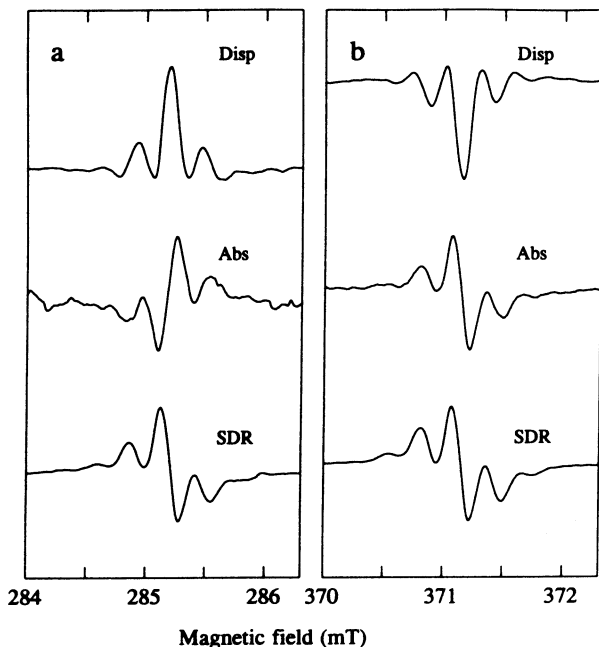
FIG. 5. Low- (a) and high- (b) field lines of Si-PT1 detected under conditions of the conventional EPR, in dispersion and absorption modes, and by microwave photoconductivity changes. Gain for EPR signals is 10^3 times higher than for SDR. EPR signals were detected with a microwave power at the level of \approx 10 \mu\text{W} , the power level for the SDR signal is \approx 1 \text{ mW} . \vec{B} \parallel \langle 111 \rangle , T=15 \text{ K} , \nu=9.213558 \text{ GHz} .
