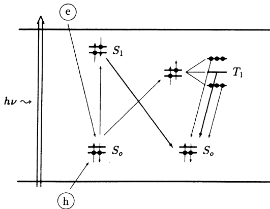
FIG. 1. Processes of the photoexcited carriers recombination via a hypothetical deep-level defect in silicon (see text for details).
