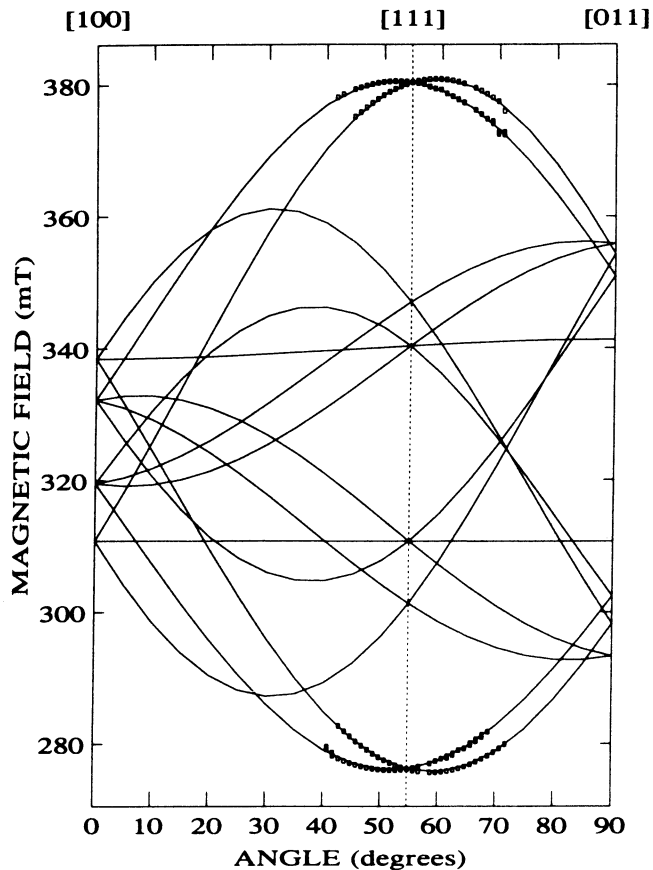
FIG. 8. Angular dependence of resonance field of the Si-PT4 spectrum. \square , experiment; solid lines, computer fit. T=15 K, \nu=9.2163 GHz.
