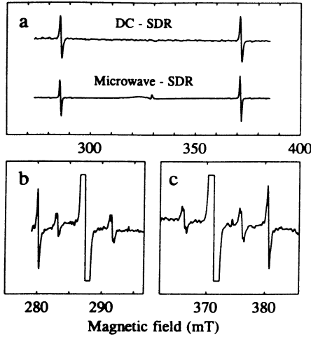
FIG. 2. EPR spectra in electron-irradiated silicon. (a) spectrum Si-PT1, detected by dc- and microwave-photoconductivity variations; (b) and (c): enlarged parts of spectrum Si-PT1 with ^{29}\text{Si} hyperfine satellites. Sharp lines at 280 and 381 mT belong to the spectrum Si-PT4.
