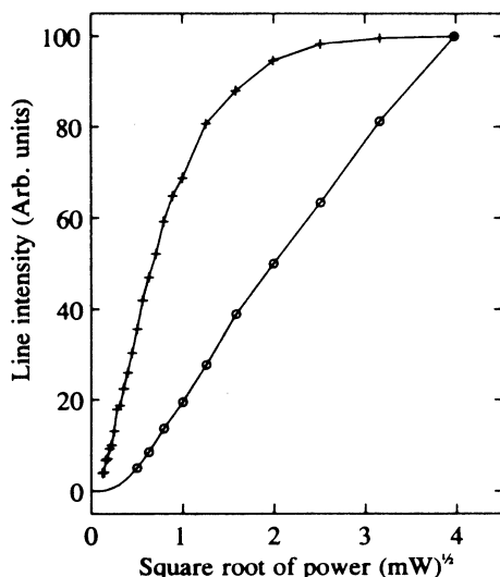
FIG. 4. Saturation curves of the Si-PT1 low-field spectrum line, detected by means of the microwave- ( \circ ) and dc- (+) photoconductivity variations. \vec{B} \parallel \langle 111 \rangle , T=15 K, \nu = 9.213648 GHz.
