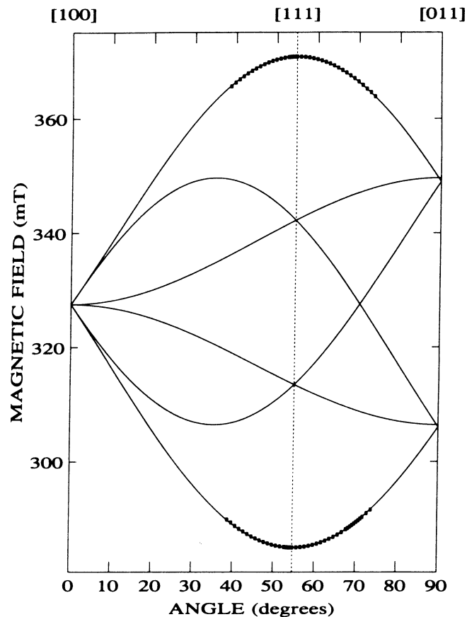
FIG. 6. Angular dependence of resonance field of the Si-PT1 spectrum. \square , experiment; solid lines, computer fit. T=15 \text{ K} , \nu=9.213648 \text{ GHz} .
