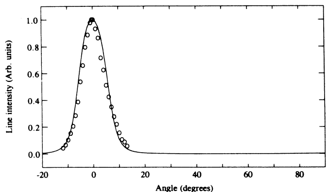
FIG. 9. Angular dependence of the Si-PT1 SDR spectrum line intensity. \circ , experiment; solid line, computer simulation. The values of the parameters are n_D = 1 \times 10^{14} \text{ cm}^{-3} , n_e = 3.4 \times 10^8 \text{ cm}^{-3} , \sigma = 1 \times 10^{-8} \text{ cm}^3 \text{ s}^{-1} , G = 1 \times 10^{13} \text{ cm}^{-3} \text{ s}^{-1} , \mathcal{R} = 2 \times 10^3 \text{ s}^{-1} , B/C = 1 \times 10^{-4} , W/C = 9 \times 10^{-2} .
