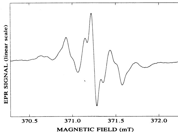
FIG. 7. Detailed scan of the high-field Si-PT1 spectrum line, taken by means of microwave-detected SDR. \nu = 9.216294 \text{ GHz} , T=15 \text{ K} .
