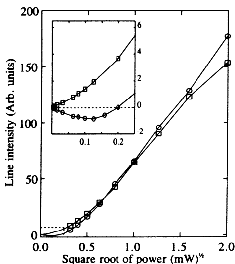
FIG. 3. Line intensity dependence of the Si-PT1 microwave-detected SDR spectrum on the microwave power. \circ , low-field line; \square , high-field line. \vec{B} \parallel \langle 111 \rangle , T=15 K, \nu = 9.213648 GHz.
